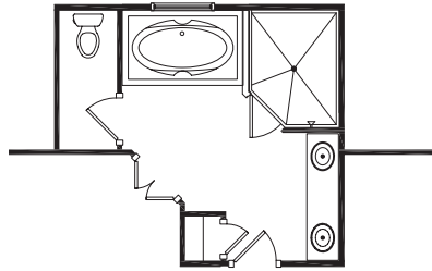
OPTIONAL MASTER BATH #1
